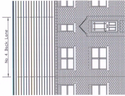
NORTH ELEVATION scale 1:100 (Existing)
